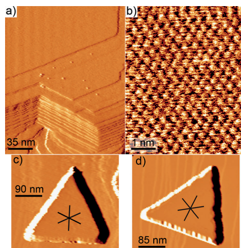
Figure 4. STM images showing the orientation of the Cu steps during Cu deposition. a) Cu steps during deposition. The angle between the steps is 120^\circ . b) Cl ^- adlayer on a Cu crystallite imaged after deposition. c) and d) show zoom-out images of the pre-deposited Cu(111) crystallites, on the surface of which (a) and (b) were acquired respectively. The black lines in (c) represent the orientations of the steps in (a) and the black lines in (d) the main symmetry axes of the Cl ^- overlayer in (b). The angle between the black lines and the side faces of the Cu crystallites is approximately 30^\circ . Images (a), (c), and (d) are differentiated.
